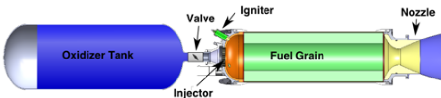
Schematic of a hybrid rocket propulsion system
